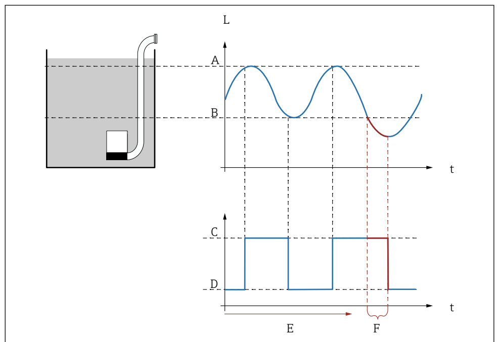
图 62 “Backlash interval”和“Backlash time”的影响
